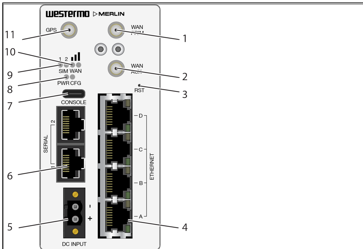
Figure 1. Location of interface ports and LEDs, illustrated by a Merlin-4407-T4-S2-LV model
