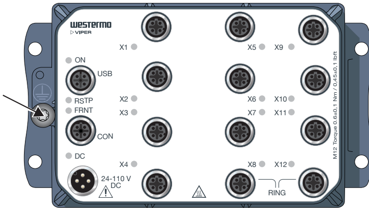
Figure 6. Earth connection
