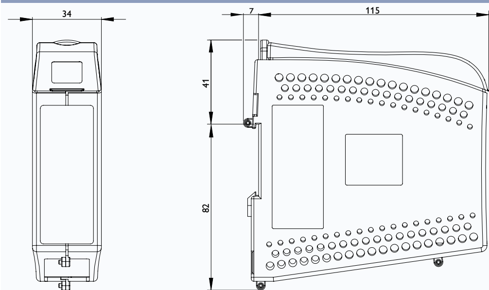
Dimensional drawing
