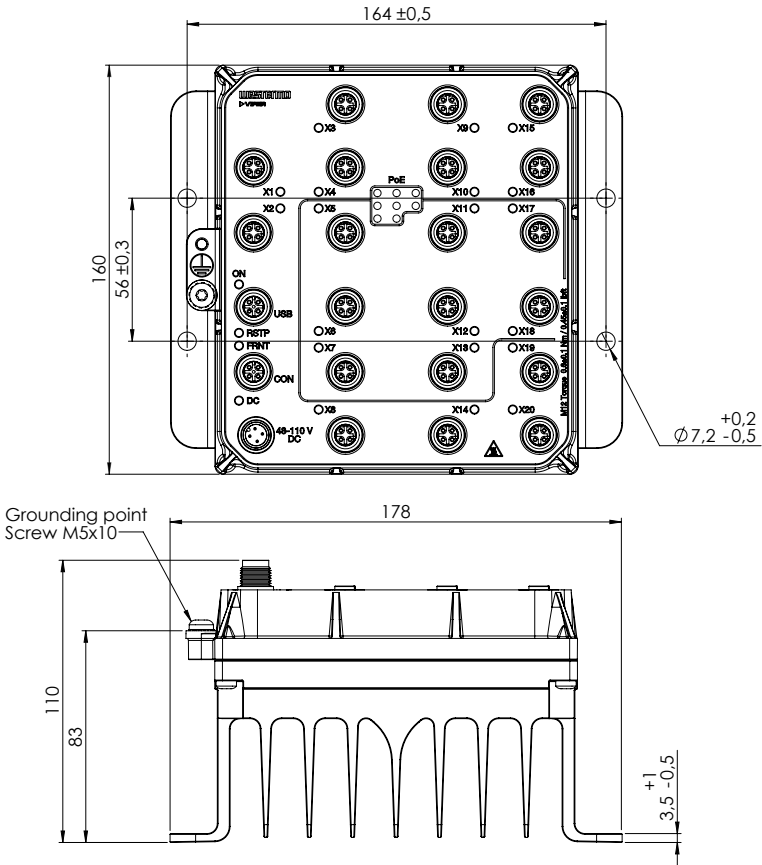
Figure 4. Dimensional drawing
