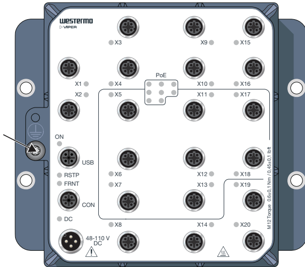
Figure 6. Earth connection
