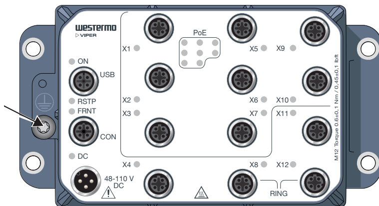
Figure 6. Earth connection
