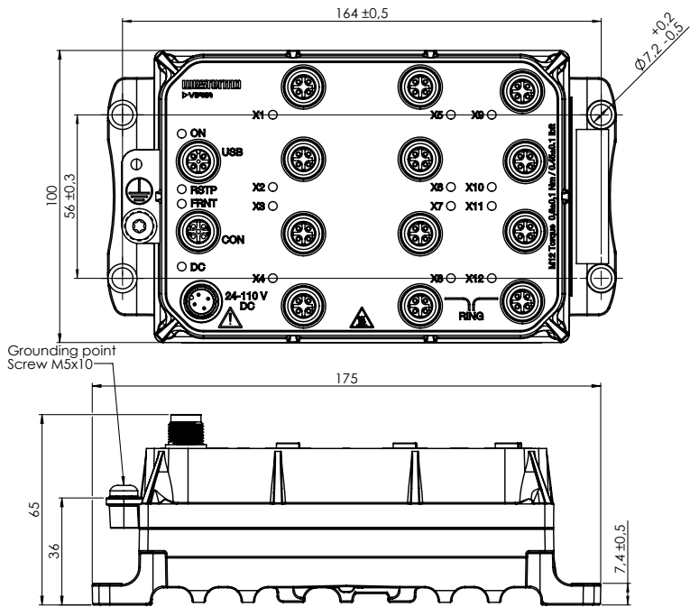
Figure 4. Dimensional drawing
