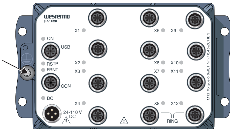
Figure 6. Earth connection
