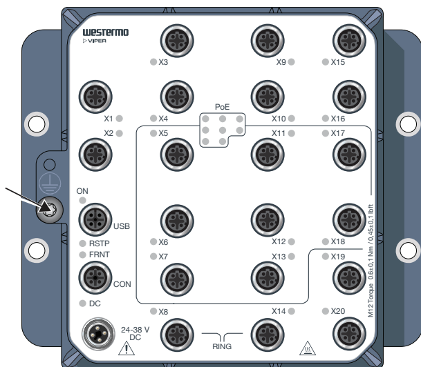
Figure 8. Earth connection
