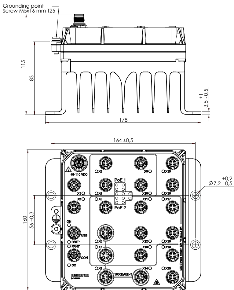
Figure 6. Dimensional drawing Viper-3520(-E)-T2G-P2G-T6-P10-HV
