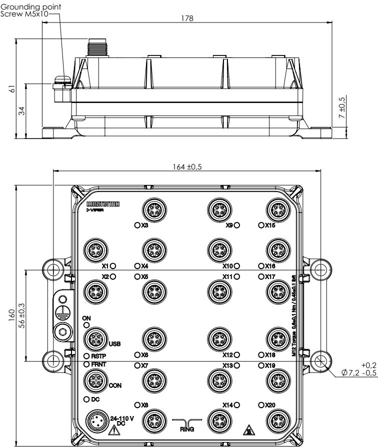
Figure 4. Dimensional drawing
