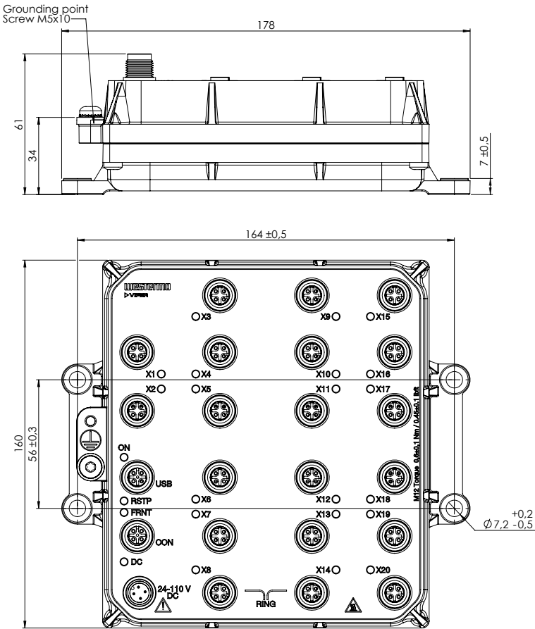
Figure 4. Dimensional drawing
