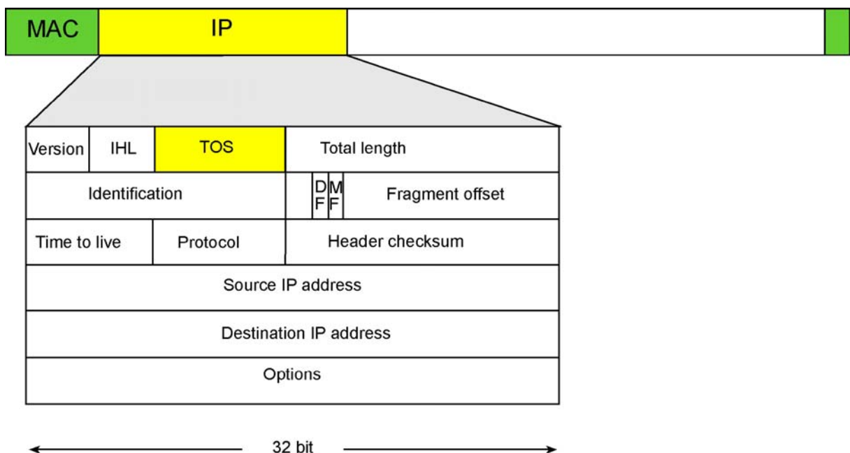
Figure 9, IP header
