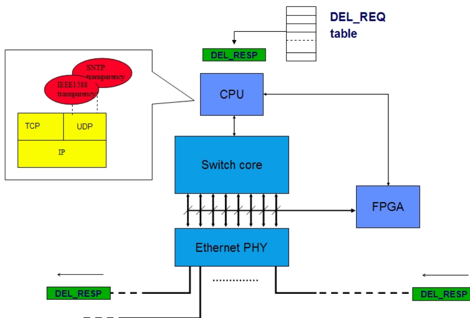
Figure 17, IEEE1588 DEL_REQ/DEL_RESP Transparent Clock functionality
