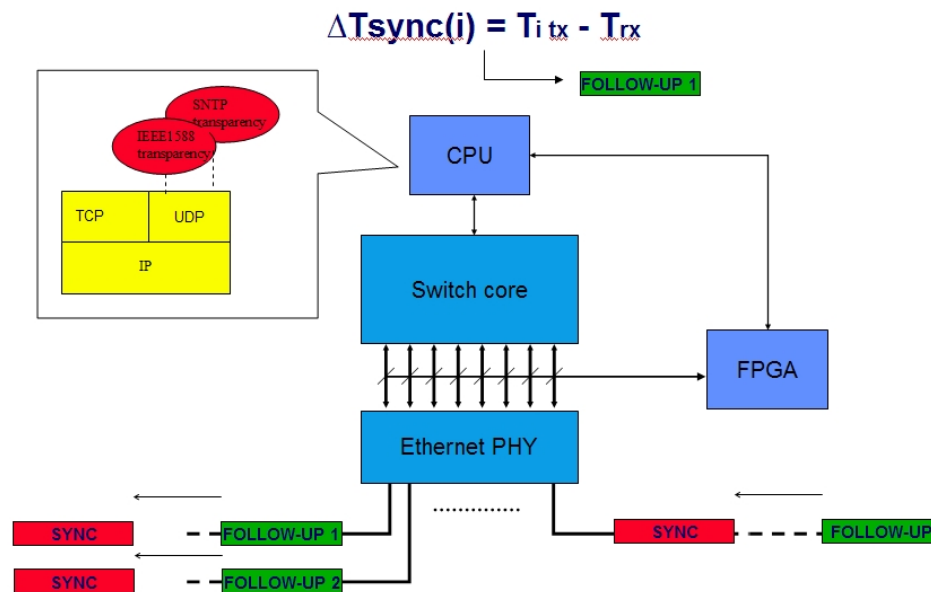
Figure 16, IEEE1588 SYNC/FOLLOW-UP Transparent Clock functionality
