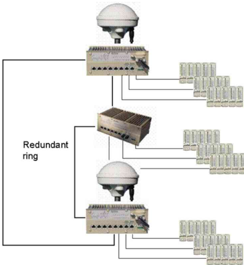
Figure 20, Network and time synchronization redundancy 1
