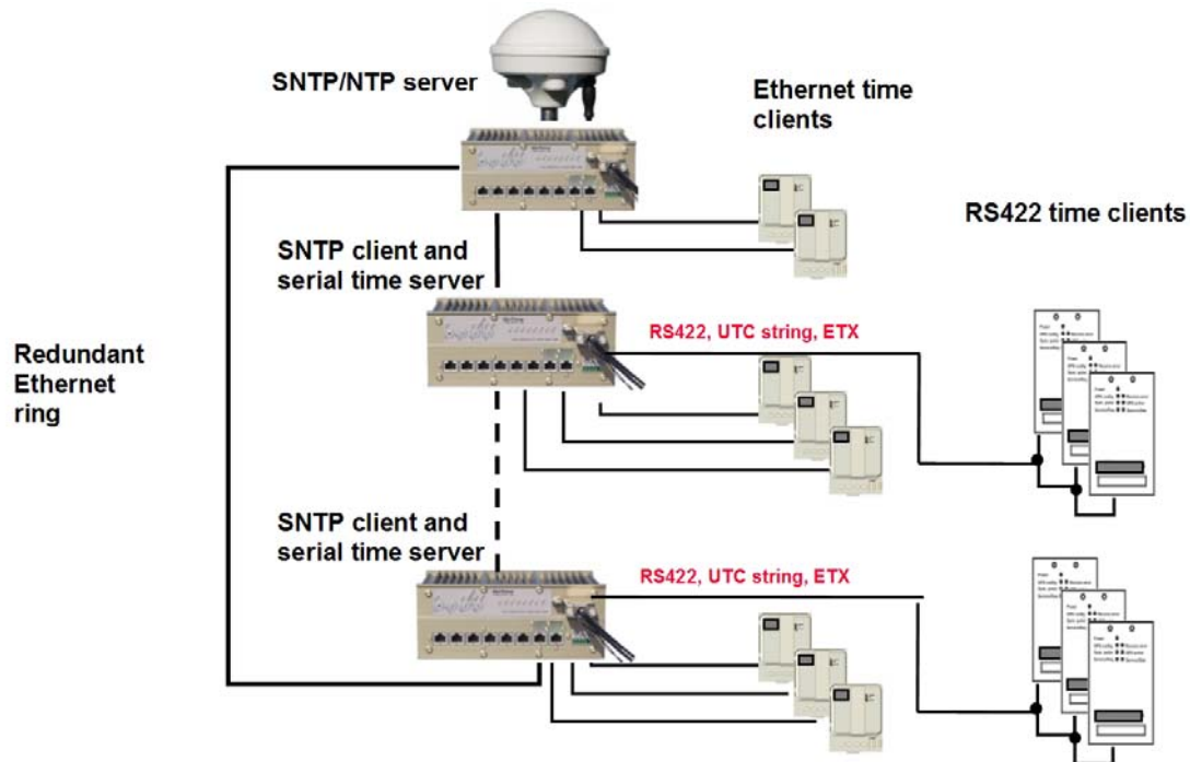
Figure 18, SNTP time client and serial time server
