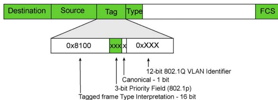
Figure 8, MAC header with tag
