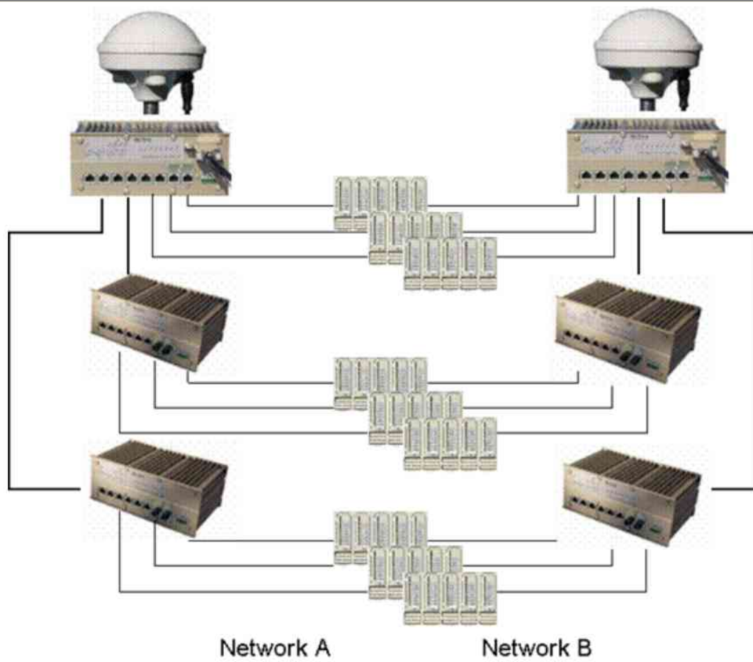
Figure 21, Network and time synchronization redundancy 2
