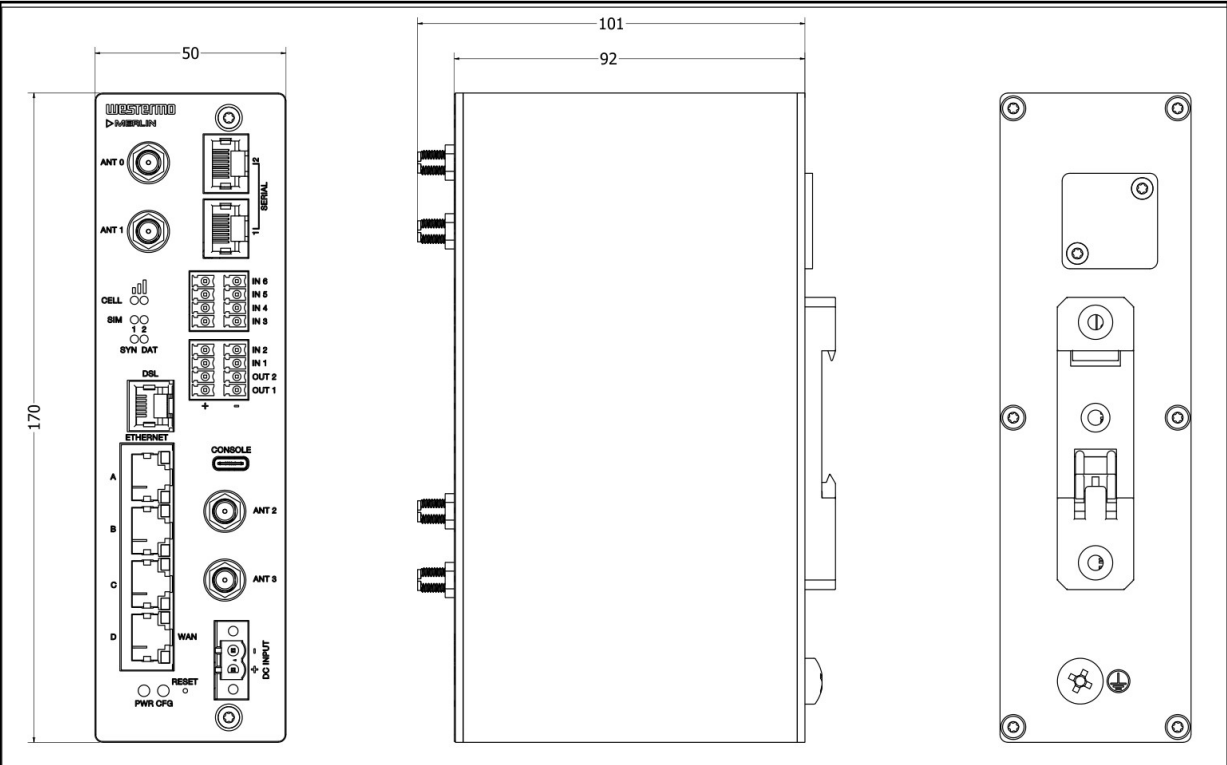
Figure 2. Dimensional drawing
