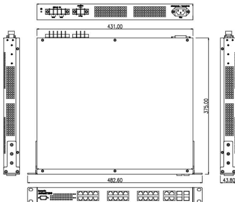
Diagram: MRI-128-F4G-PSE/24
