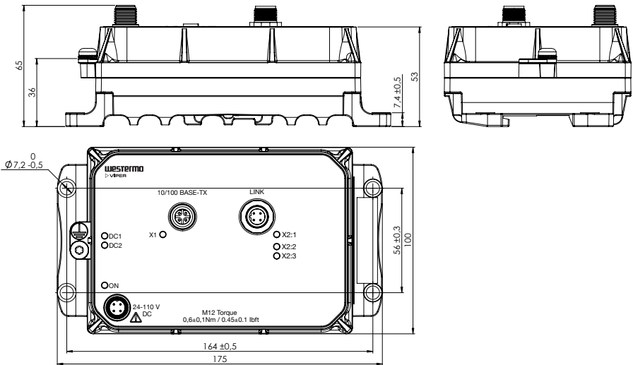
Figure 5. Dimensional drawing
