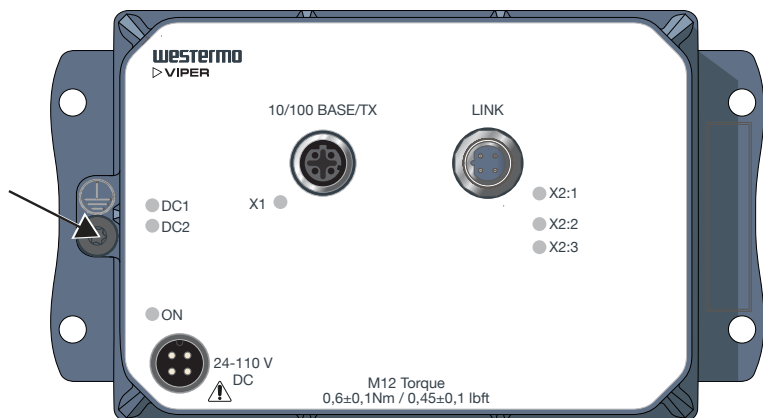
Figure 7. Earth connection
