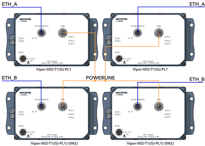
Figure 3. Explanatory overview
