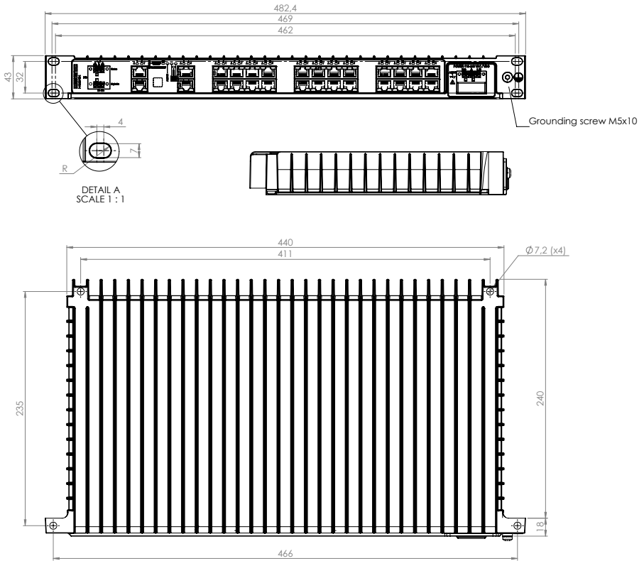
Figure 5. Dimensional drawing
