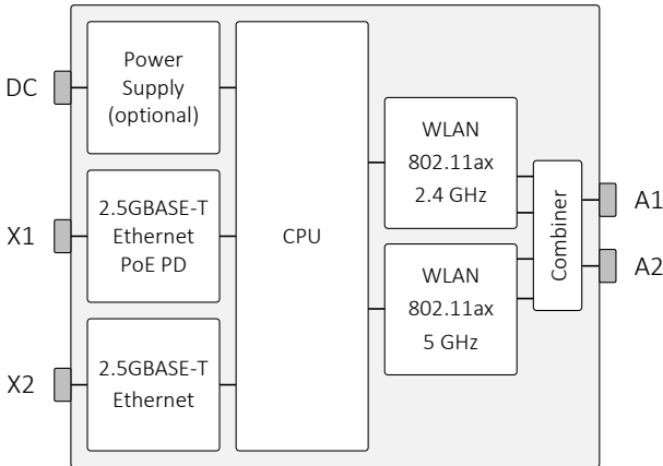
Figure 4. Ibex-1310 block diagram
