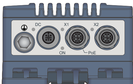
Figure 5. LED indicators
