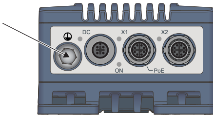
Figure 7. Earth connection
