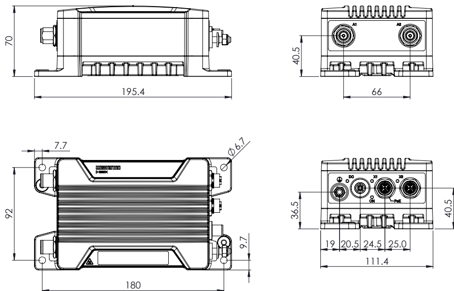
Figure 6. Dimensional drawing
