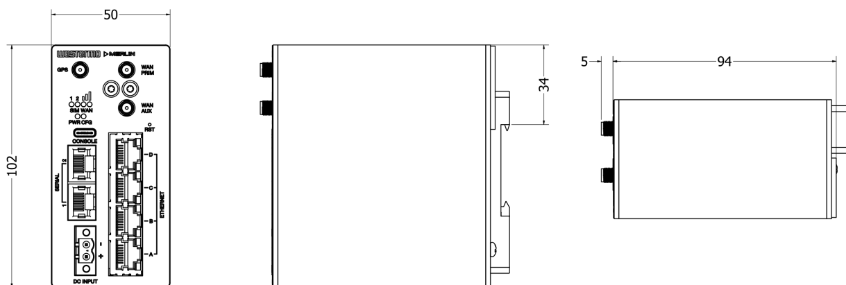
Figure 7. Dimensional drawing
