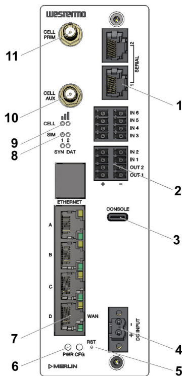
Figure 3. Location of interface ports and LEDs, illustrated by a Merlin-4707-T4G-S2-DI6-DO2-LV model
