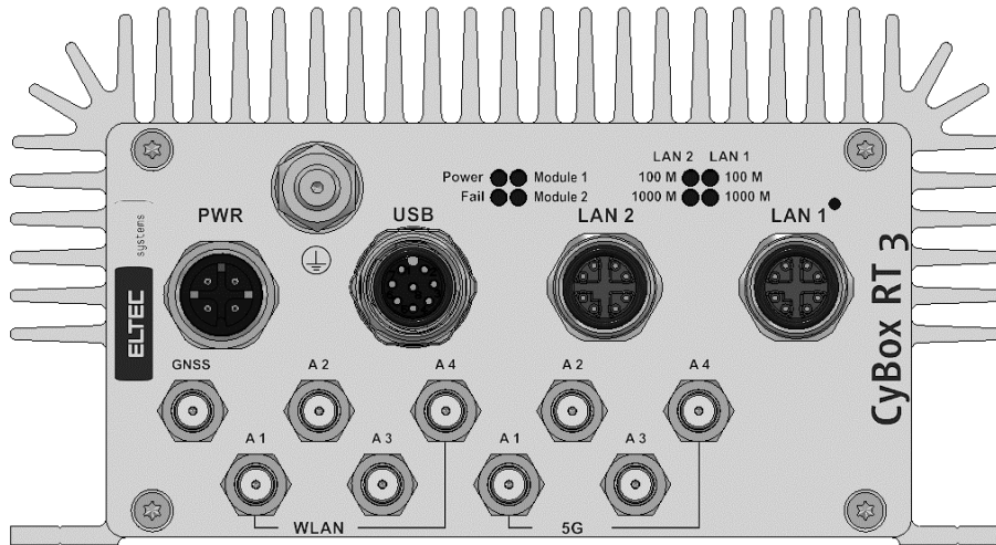
Figure 3 Frontblenden-Überblick
